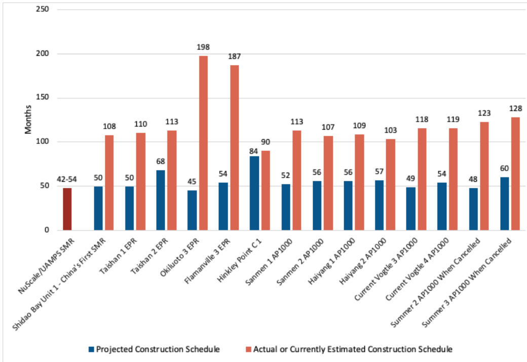
Figure 2: Recent Nuclear Construction Schedules for Nuclear Plants With New Designs 26
