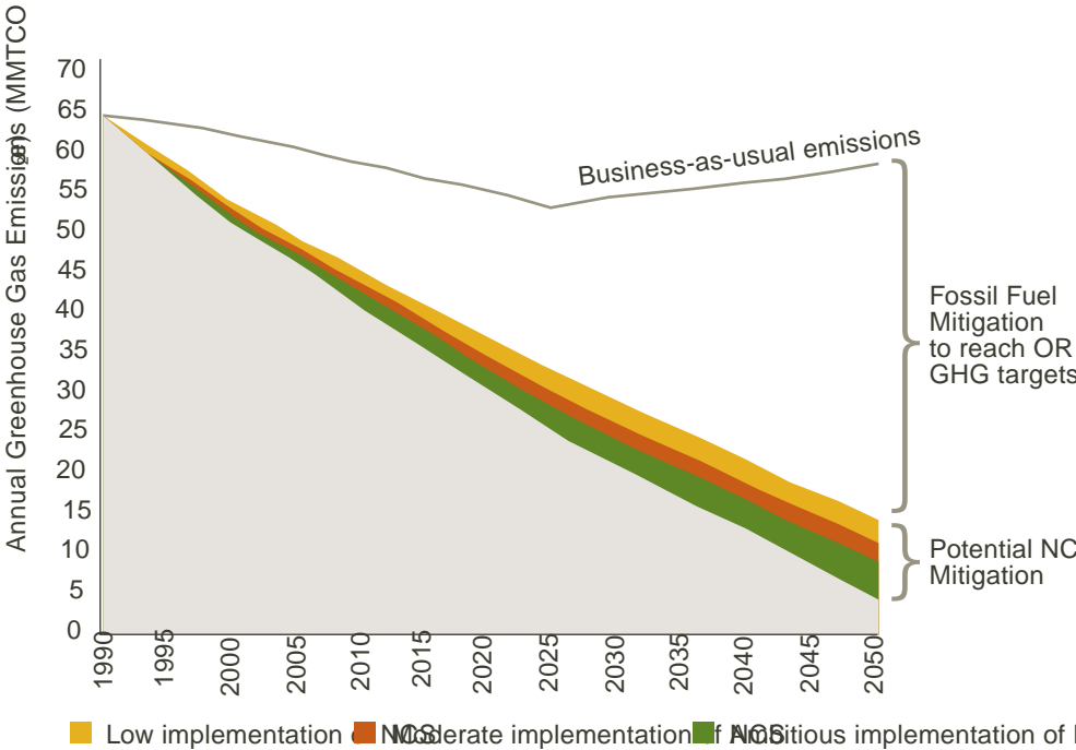
This figure illustrates NCS potential relative to Oregon's 2018 projected business-as-usual emissions trajectory and state 2050 statutory goal. The white area shows the needed fossil fuel mitigation across other sectors while the colored wedges show the potential contribution of NCS. Modified from Graves et al. 2020.
