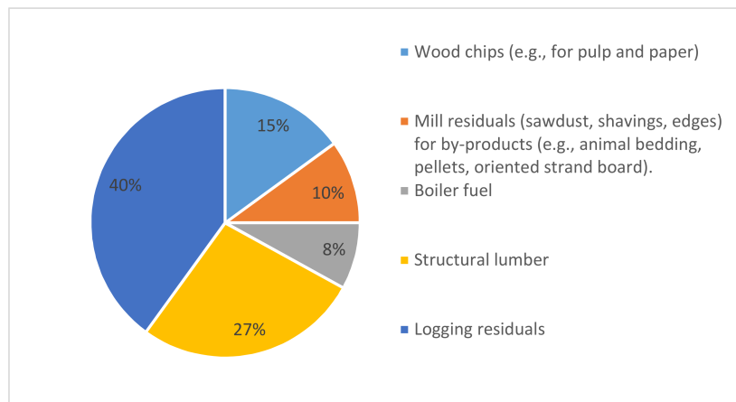
Figure 2. Tree biomass (Douglas fir) division upon harvest [23].
