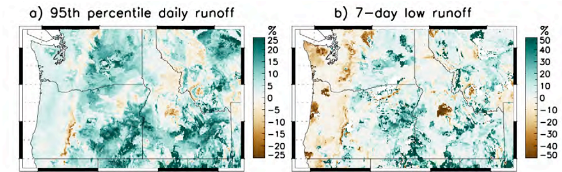
Figure 3.3 Percentage change in mean (a) high runoff (the 95th percentile of daily total runoff) and (b) low runoff (7-day average lowest flow per year). Changes are for 2011–2050 under the high (RCP 8.5) emissions pathway relative to 1966–2005. The 95th percentile runoff and the 7-day average lowest flows were averaged over 11 CMIP5 models prior to calculating changes (Figure source: David Rupp; data source: Naz et al. , 2016)
