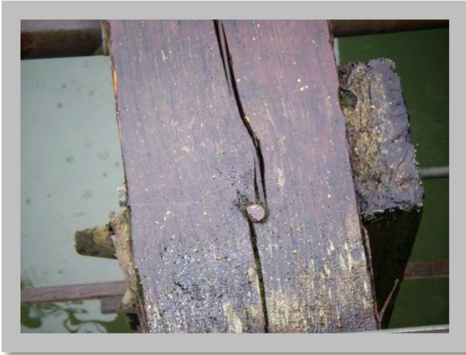
Figure 6.9: The connection on this pier in the CEI Hub appears to have deteriorated due to a split in the timber beam. This type of damage suggests that the condition of the structure may not be routinely monitored and maintained and that the overall pier is seismically vulnerable (Source: DOGAMI photo)
