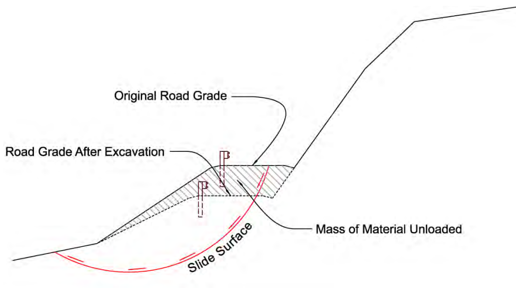
Figure 5.11: Stabilizing a landslide by the “unloading” method. (Source: ODOT – Geo-Environmental Section)
