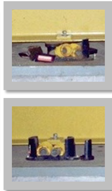
Figure 7.11a and 7.11b: Close-up of the two vibration isolation units. The cause of the failure was due to lack of details to limit the generator displacement during the strong shaking.
