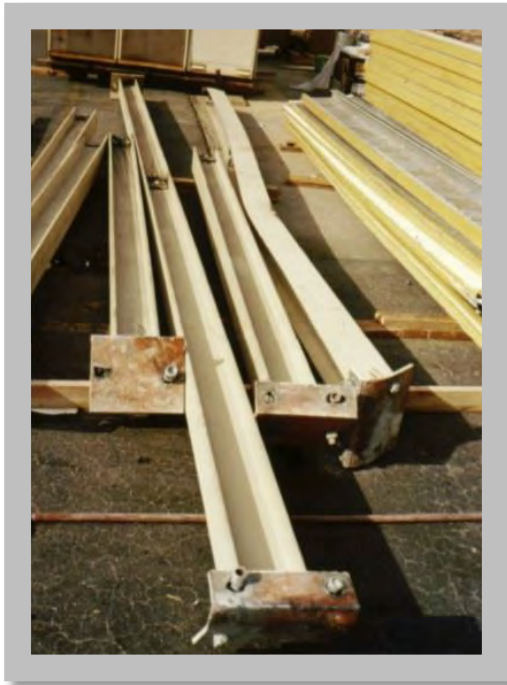
Figure 7.15 – Collection of damaged bracing beams removed from Central Office. Northridge earthquake, California, 1994. (Source: Alex Tang)
