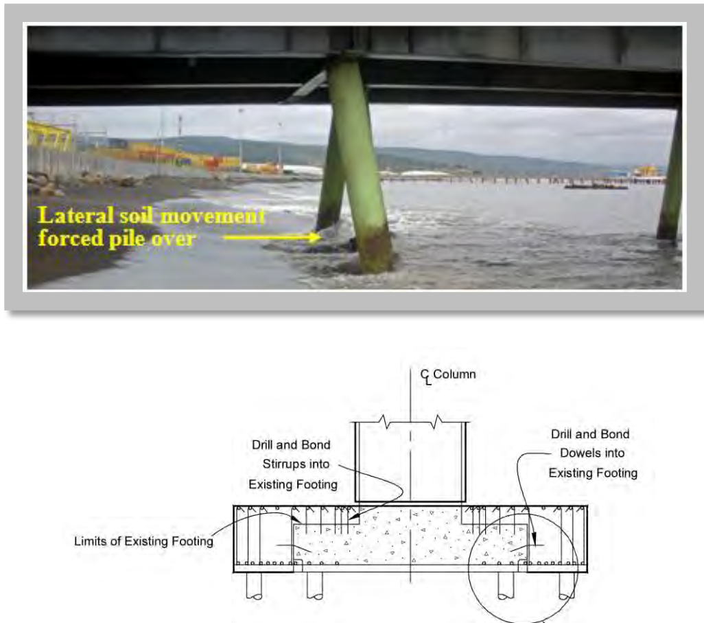
Figure 5.5: Strengthening the foundation or soil mitigation will prevent the damage to the bridge substructure due to liquefaction and lateral spreading (Photo Source: www.fhwa.dot.gov )
