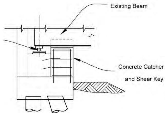
Figure 5.3: Shear Keys will restrain the superstructure transversally during an earthquake. (Photo Source: www.fhwa.dot.gov )
