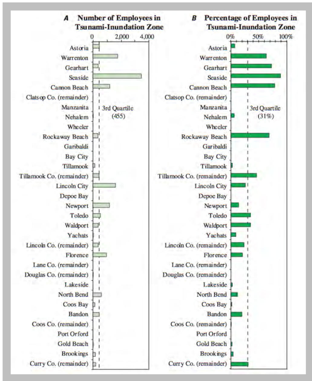
Figure 3.7: Number and Percentage of Employees in the Tsunami Inundation Zone. Wood, Nathan: 2007, Variations in City Exposure and Sensitivity to Tsunami Hazards in Oregon . (Source: US Geological Survey)
