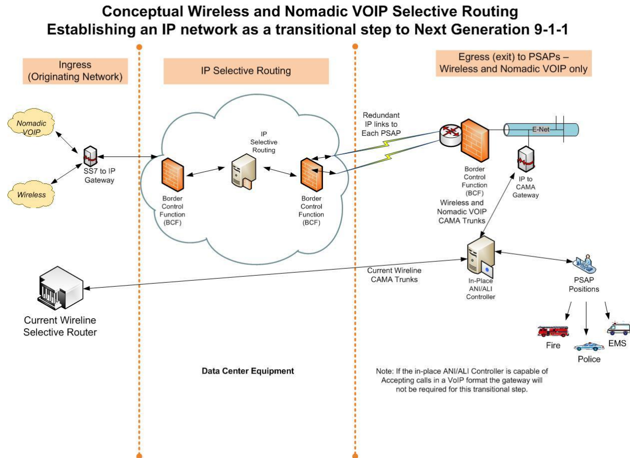
Figure 14 – Conceptual Design
